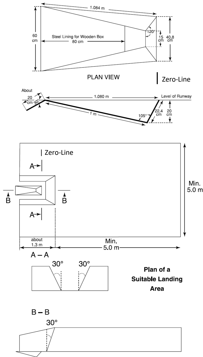
FIGURE 5 – POLE VAULT BOX AND LANDING AREA
