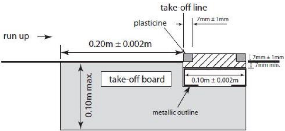
FIGURE 6 – TAKE-OFF BOARD AND PLASTICINE BOARD
